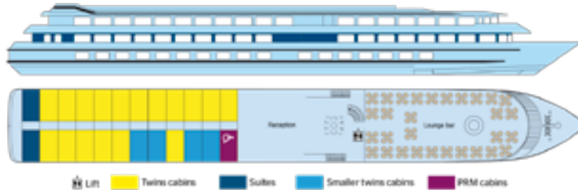
Middle Deck
